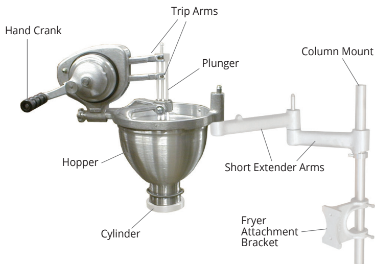
Belshaw Type N shown with column mount and short extender arms.
