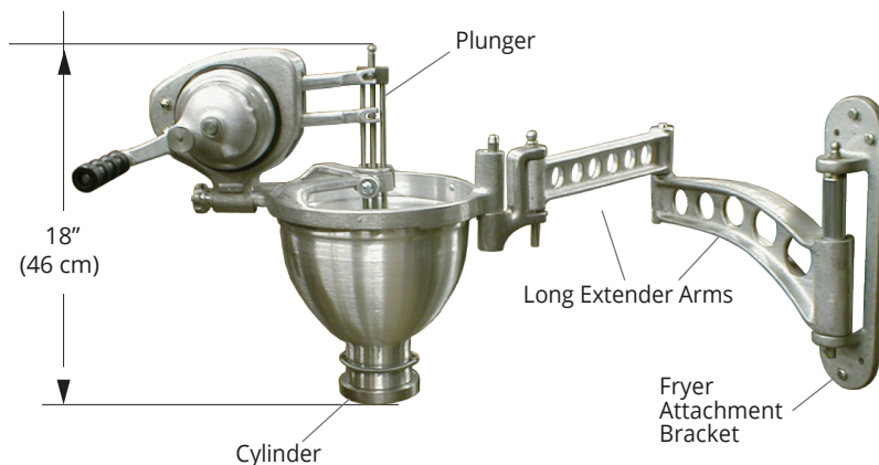
Belshaw Type N shown with wall mount and long extender arms, for bolting to a wall.
